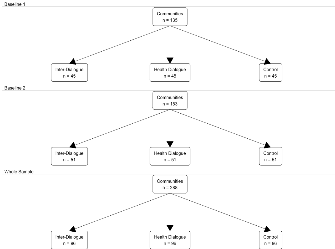
Figure 1: Treatment Assignment
