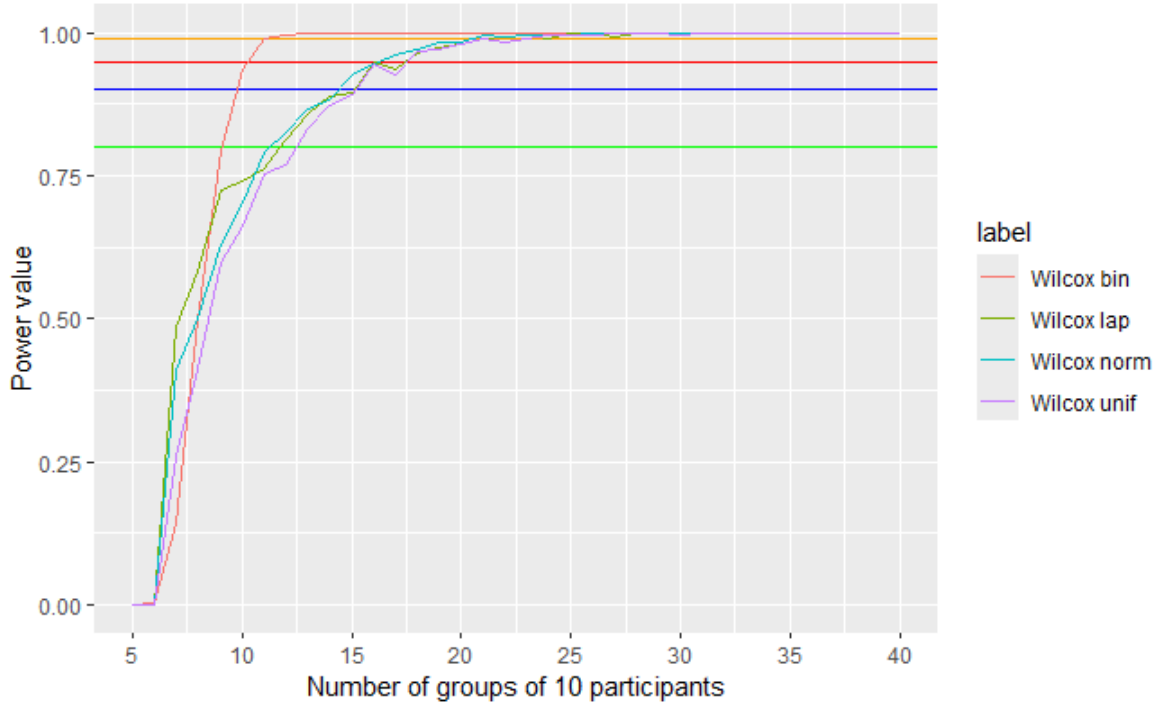
FIGURE 4 – Tests' power for a mean deviation of 2 and a standard deviation of 1.8
