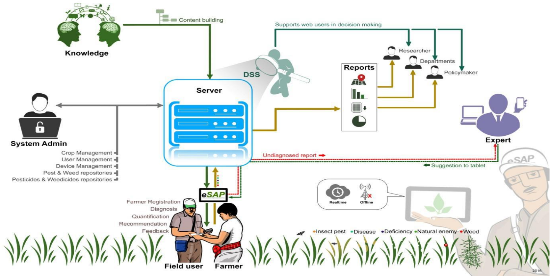
Figure 1: eSAP workflow
