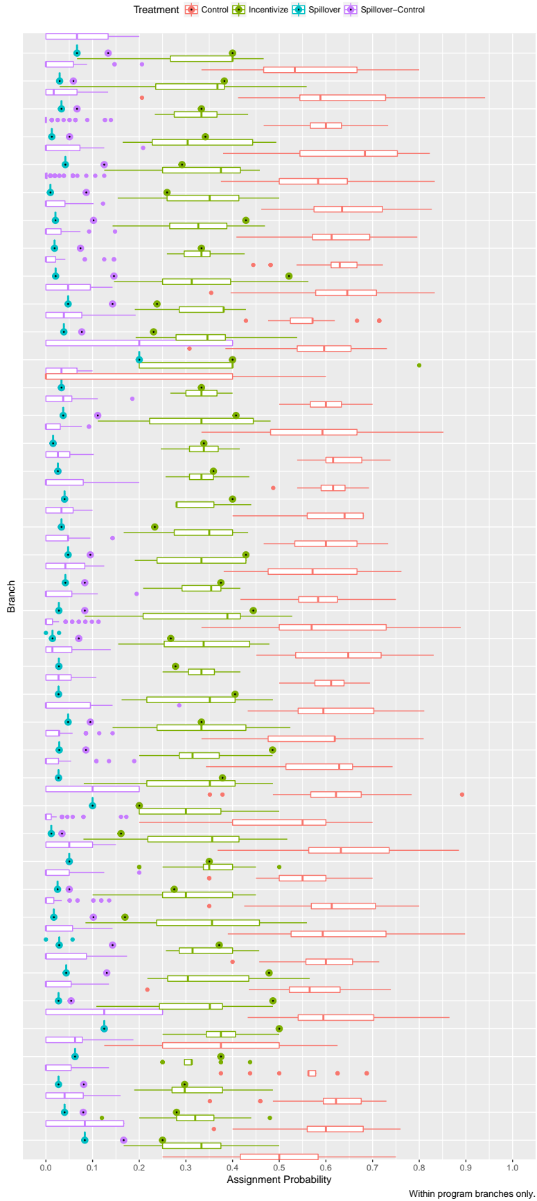
Figure 4: Treatment Assignment Probability 20
