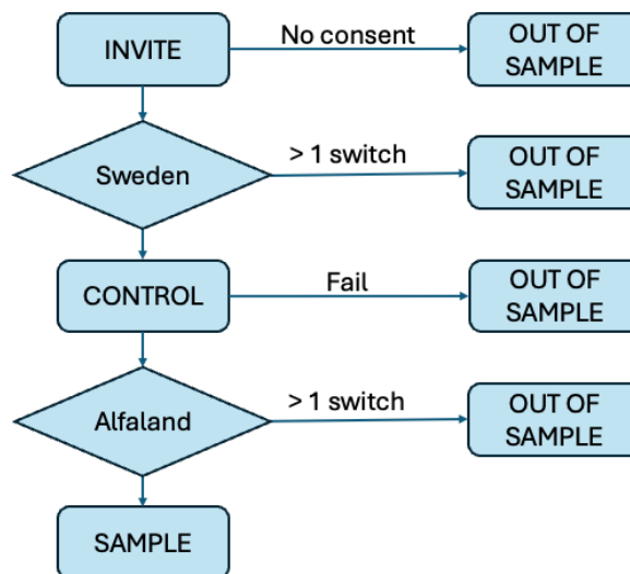
Figure 3: Simplified flowchart illustrating selection of final analysis sample
