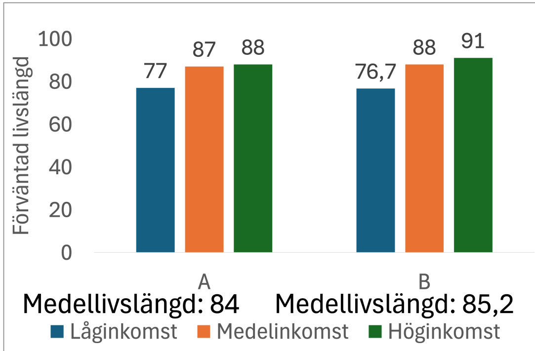
Figure 4: The choice between A and B, for \nu = 4
